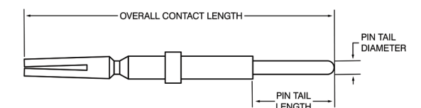
PC Tail Contact
