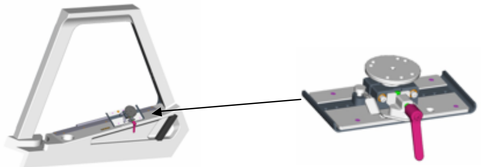
FIGURE 2: Captain's Side Window Modified With EZMount Slider (First Officer's Installation is Mirror Image)
